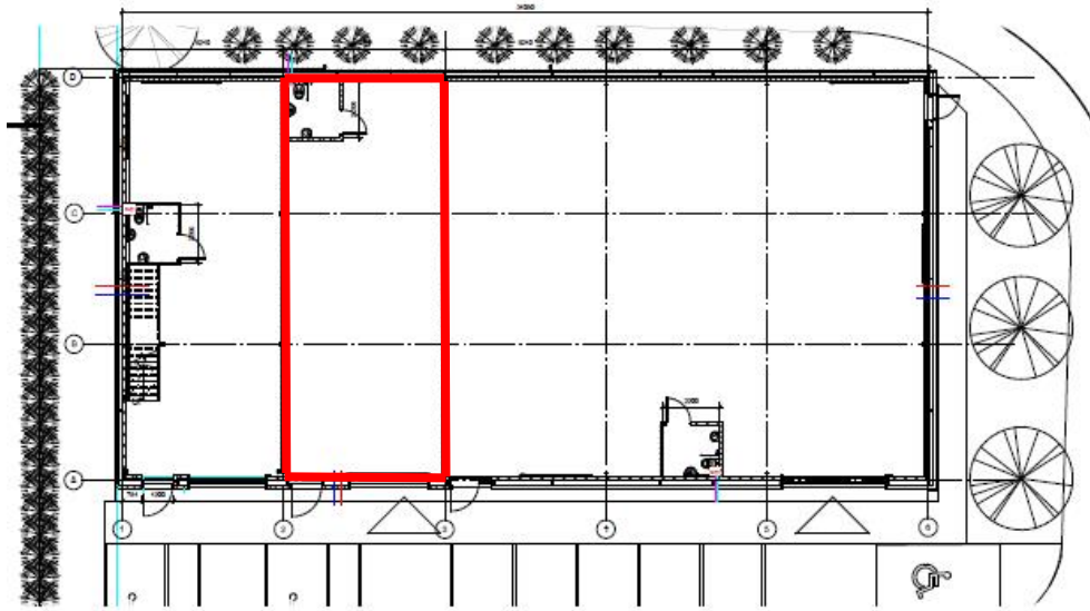
Level 0 Plan 1:100
